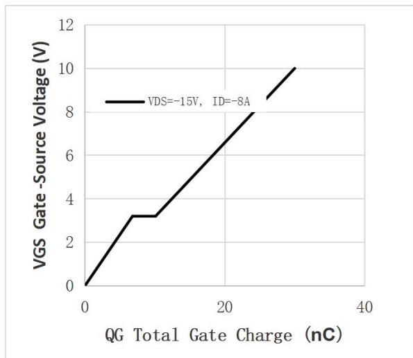
Fig.1 Gate-Charge Characteristics
