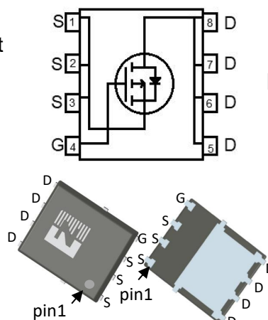
DFN5*6
